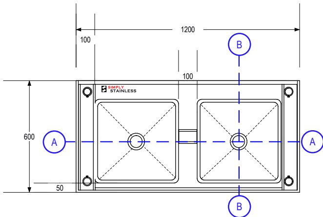
BOTTOM-PLAN VIEW (TOP ONLY)
