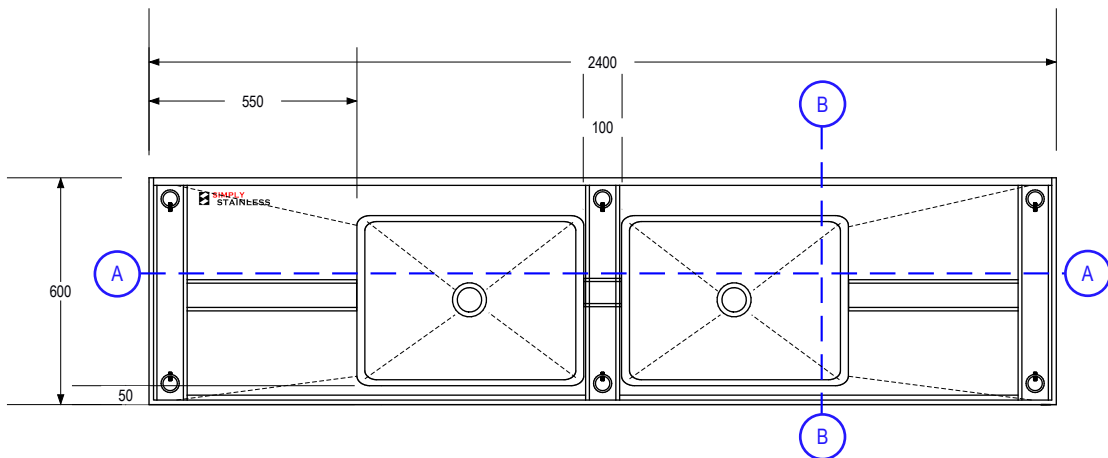
BOTTOM-PLAN VIEW (TOP ONLY)
