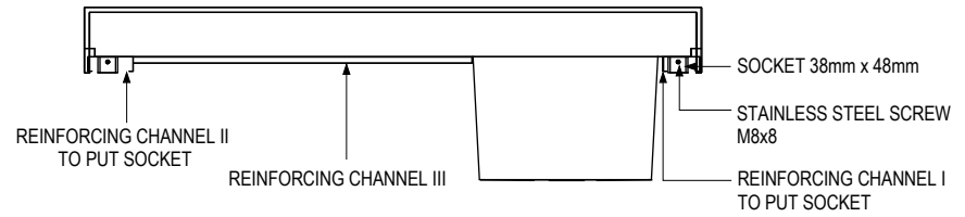
A-SECTION VIEW SCALE 1:15mm
