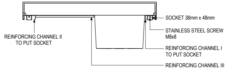
A-SECTION VIEW SCALE 1:15mm
